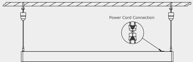
Installation Diagram
